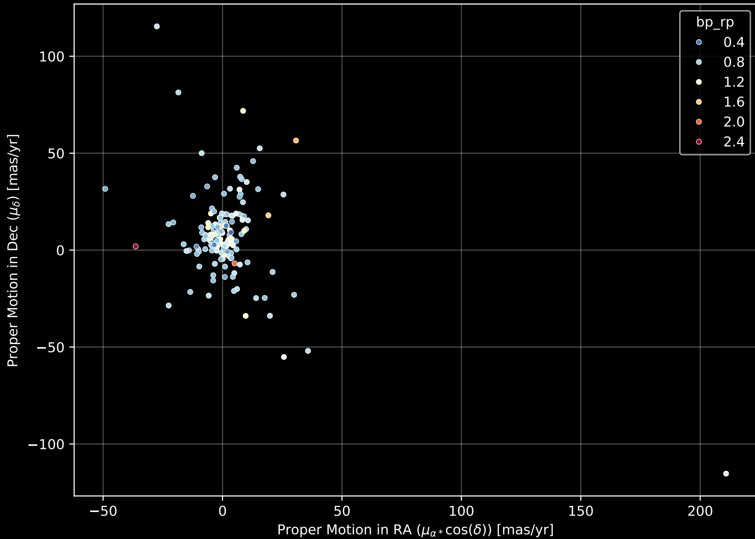
GALAH DR4 Field: [7188] Proper Motion Diagram (n= 154)
