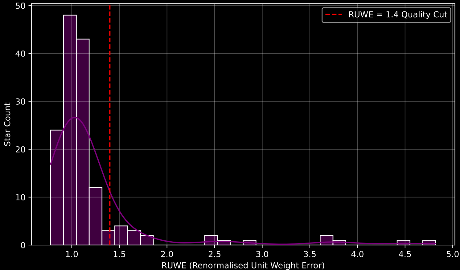
GALAH DR4 Field [7188] RUWE Distribution (n= 148)
