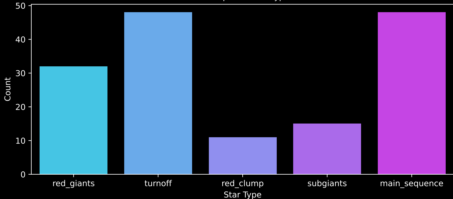
GALAH DR4 Field: [7188] Count plot of Star Type
